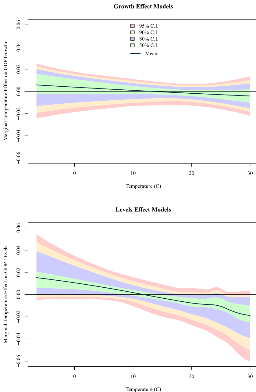
Fig. 2. Confidence regions of temperature marginal effects on \Delta \ln(GDP) (top) and \ln(GDP) (bottom). Notes: Plotted are 50, 80, 90, and 95% confidence regions of temperature marginal effects on GDP growth (top panel) and GDP levels (bottom panel). Confidence regions are determined by bootstrapped sampling 1000 times for each model specification that appears in the union of model confidence sets.
